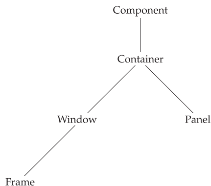
Figure 24-1 The class hierarchy for Panel and Frame
