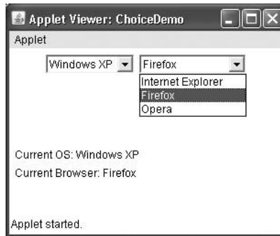
Figure 25-4 Sample output from the ChoiceDemo applet
